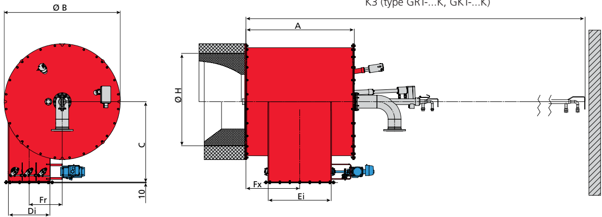
K1 (type GT...K) K2 (type RT...K, KT...K) K3 (type GRT...K, GKT...K)
