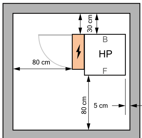
Access clearance (RE RVS) ver. 1
